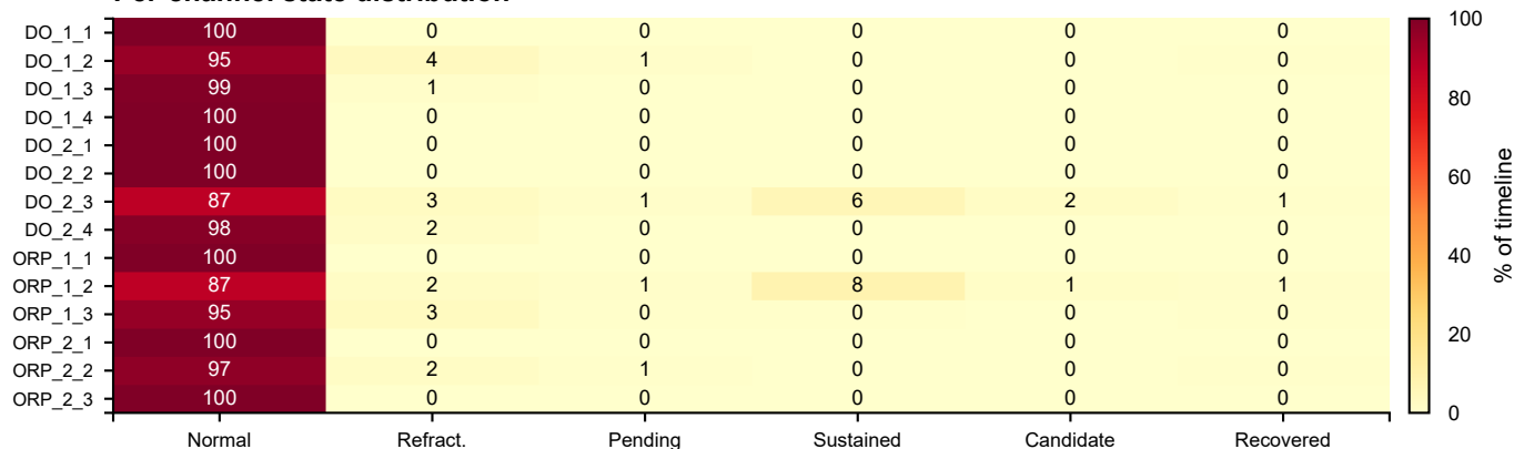
Figure V14. Six-state occupancy, transitions, and veto co-activation
